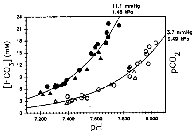
FIG. 2. A \text{pH}-\text{HCO}_3^- (i.e., Davenport) diagram for yellowfin tuna blood equilibrated to 0.5% \text{CO}_2 ( P_{\text{CO}_2} = 3.7 mmHg or 0.49 kPa) at 20°C (○) and 30°C (△), and to 1.5% \text{CO}_2 ( P_{\text{CO}_2} = 11.1 mmHg or 1.48 kPa) at 20°C (●) and 30°C (▲). [\text{HCO}_3^-] was measured in true plasma anaerobically separated at room temperature. Lines, added simply for illustrative purposes, were fitted using a nonlinear least-squares regression.
