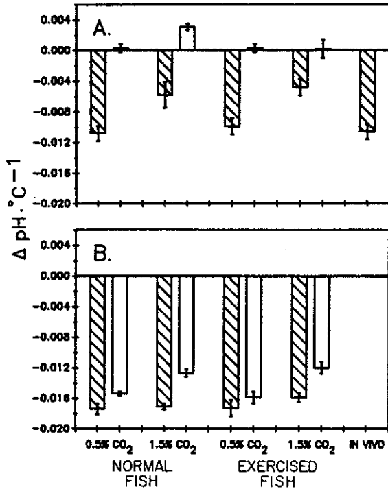
FIG. 4. Rates of pH change in vitro in true plasma (hatched bars) and separated plasma (open bars) for normal and exercised yellowfin tuna during (A) open-system (constant P_{\text{CO}_2} , variable \text{CO}_2 content) and (B) closed-system (constant \text{CO}_2 content, variable P_{\text{CO}_2} ) temperature changes. True plasma pH changes (arterial blood samples) with temperature occurring in vivo are also shown in A.
