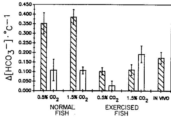
FIG. 5. Effects of in vitro open-system temperature changes on [\text{HCO}_3^-] of true plasma (hatched bars) and separate plasma (open bars) from normal and exercised yellowfin tuna. The effects of in vivo temperature changes on true plasma [\text{HCO}_3^-] (in arterial blood samples) are also shown.
