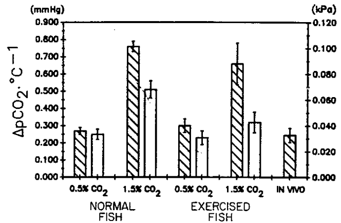
FIG. 6. Effects of closed-system temperature changes on P_{\text{CO}_2} of whole blood (hatched bars) and separated plasma (open bars) from normal and exercised yellowfin tuna. P_{\text{CO}_2} changes in arterial blood occurring in vivo are also shown.
